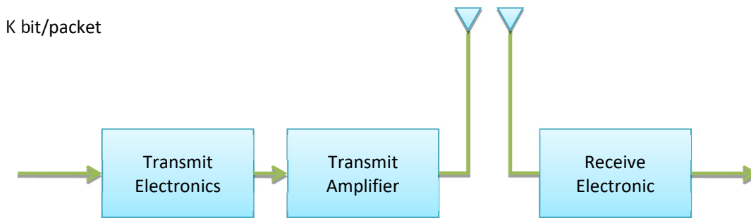
Fig1. Network Model
