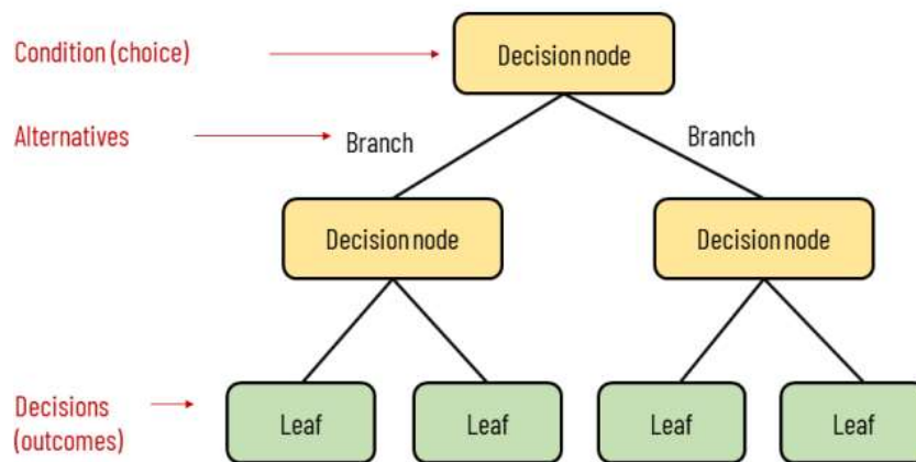
Figure 1.3 Decision Tree
