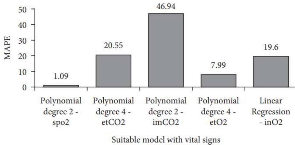
Figure 1.6 Best regression models for 60-second forecasted vital signs.
