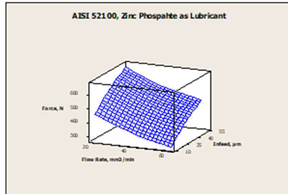
Fig. 8. AISI 52100, Zinc Phosphate as lubricant
