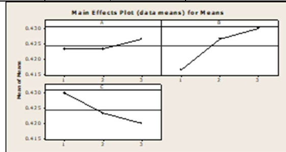
Fig. 10 Main Effects Plot (data means) for Means for Zinc Phosphate
