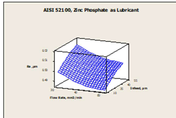
Fig. 13. AISI 52100, Zinc Phosphate as lubricant
