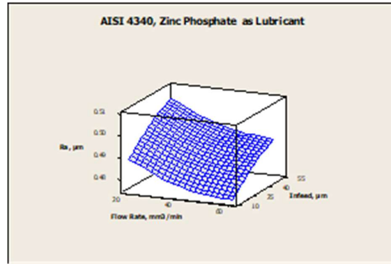
Fig. 12. AISI 4340, Zinc Phosphate as lubricant
