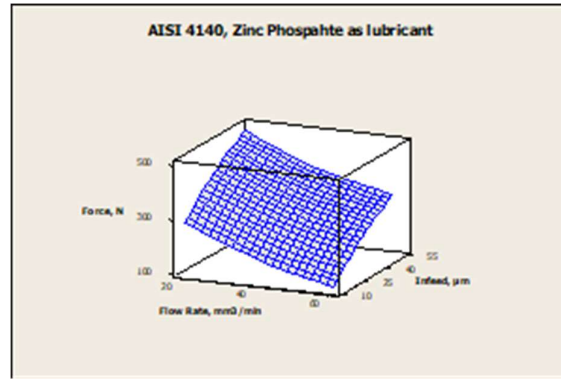
Fig. 6. AISI 4140, Zinc Phosphate as lubricant
