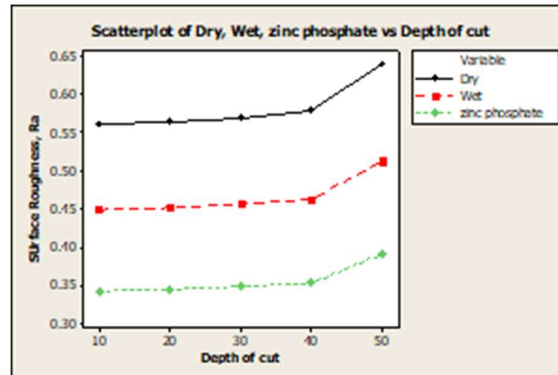
Fig. 3. Surface roughness for AISI 4140 using different coolants.
