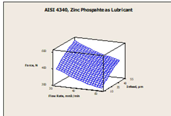
Fig. 7. AISI 4340, Zinc Phosphate as lubricant
