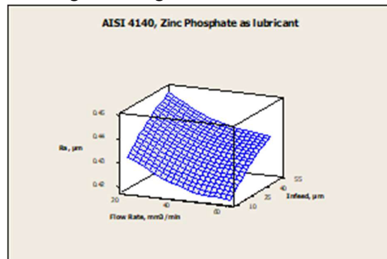
Fig. 11. AISI 4140, Zinc Phosphate as lubricant
