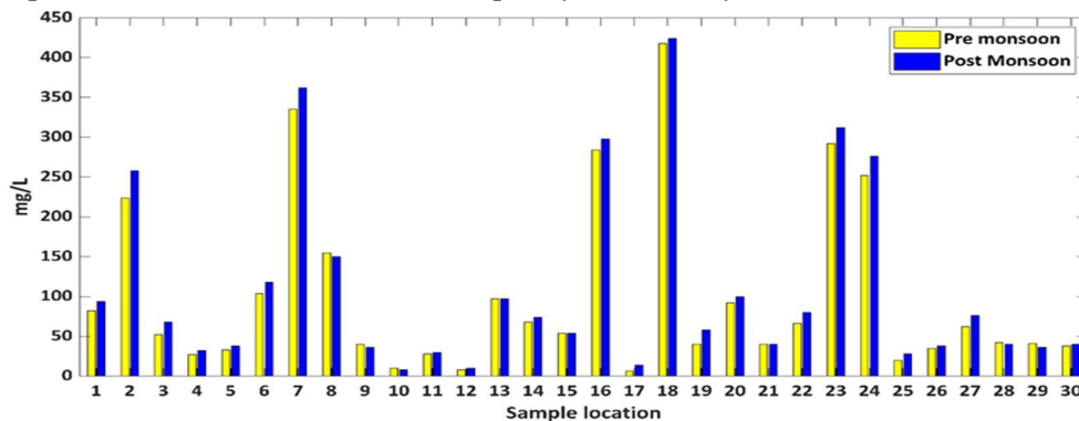
Figure 2. NO 3 Concentration in water at different sample locations
