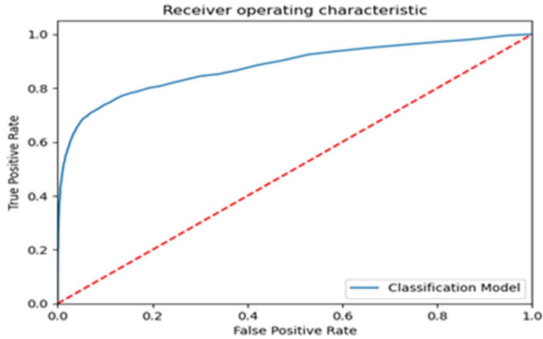
Fig.4. Analysis of Random Forest Classifier
