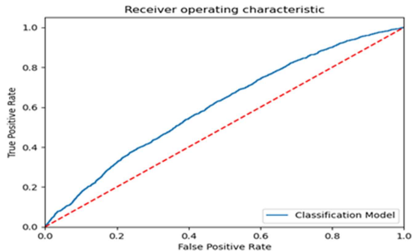
Fig.2. Analysis of Logistic Regression
