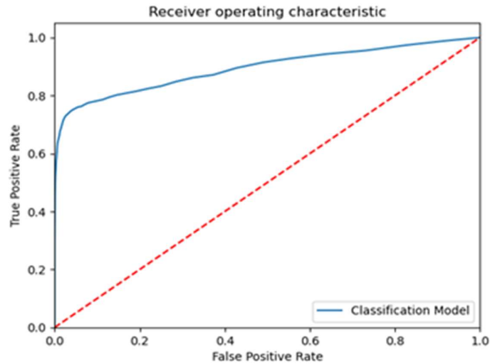
Fig.7. Analysis of Extra Trees Classifier
