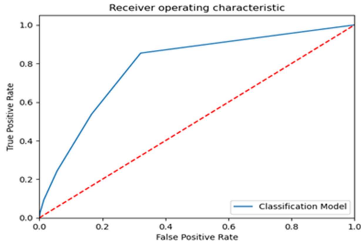
Fig.6. Analysis of KNeighbors Classifier
