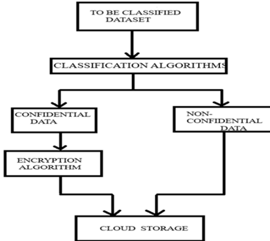
Fig.1.Proposed Mechanism
