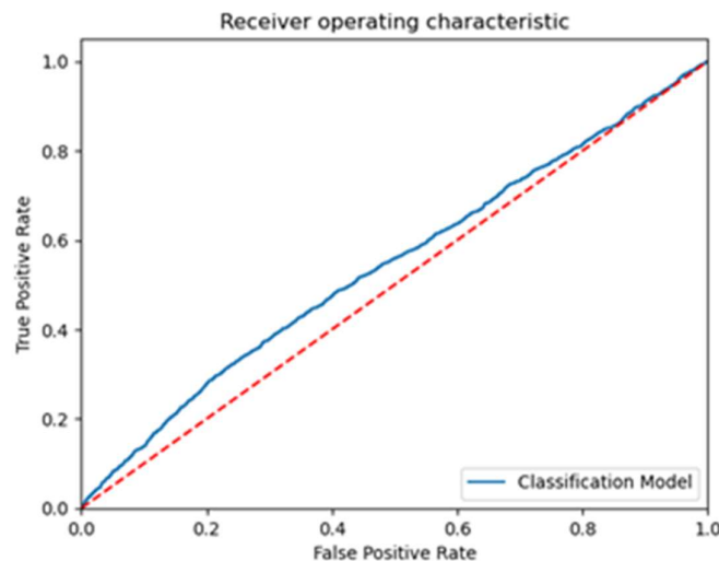
Fig.5. Analysis of Gaussian NB
