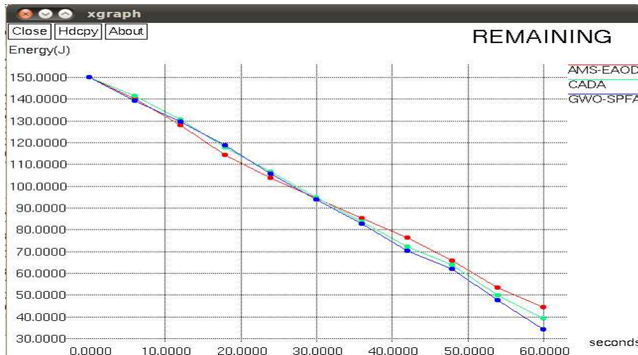
Figure 4.4: Energy consumption comparison
