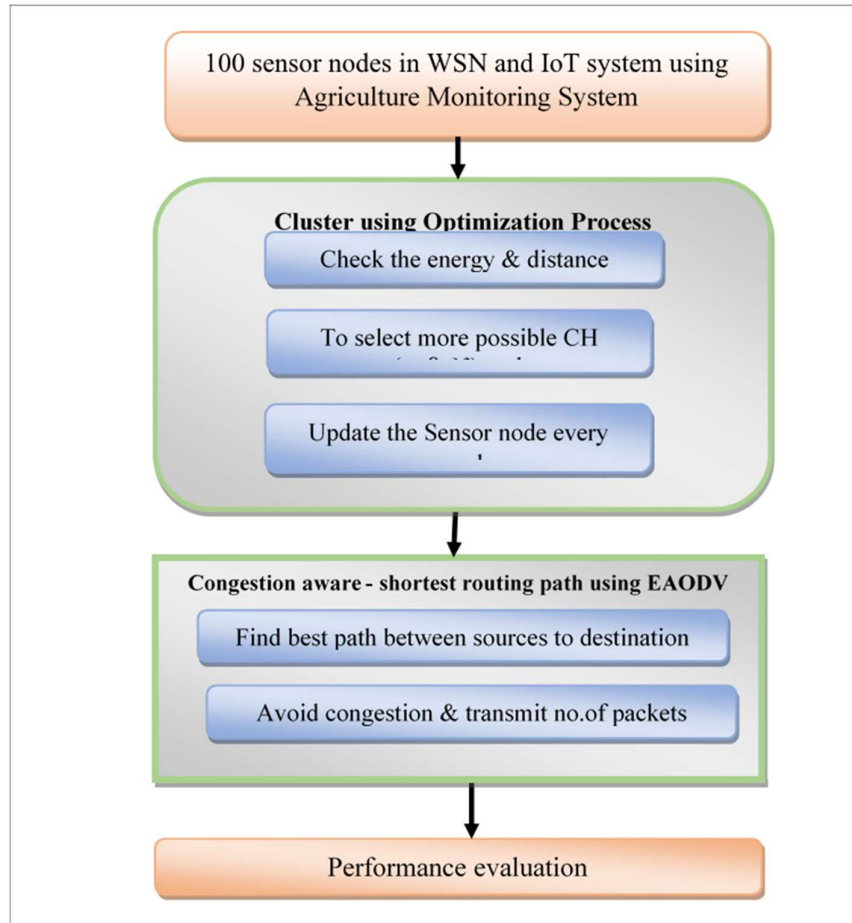
Figure 2: Architecture of ACM EAODV using IOT and WSN
