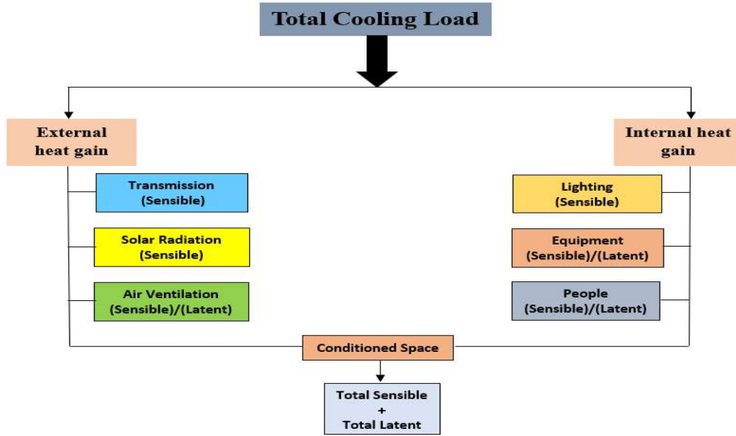
Fig. 2: Components of Cooling load in Building
