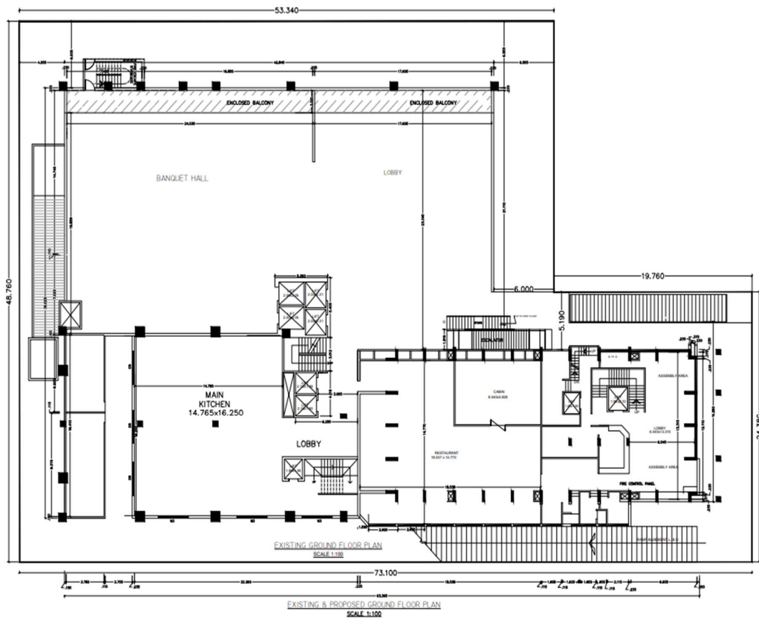
Fig. 5: Building Ground Floor Plan
