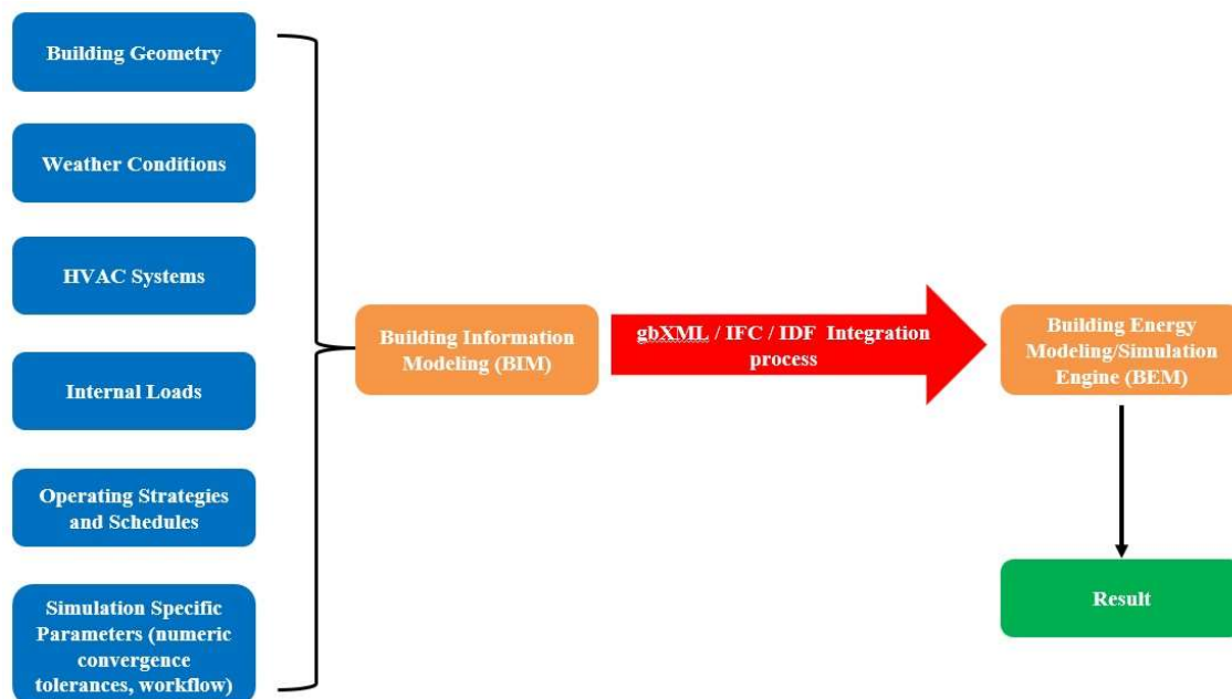
Fig. 1: BIM-BEM simulation flow
