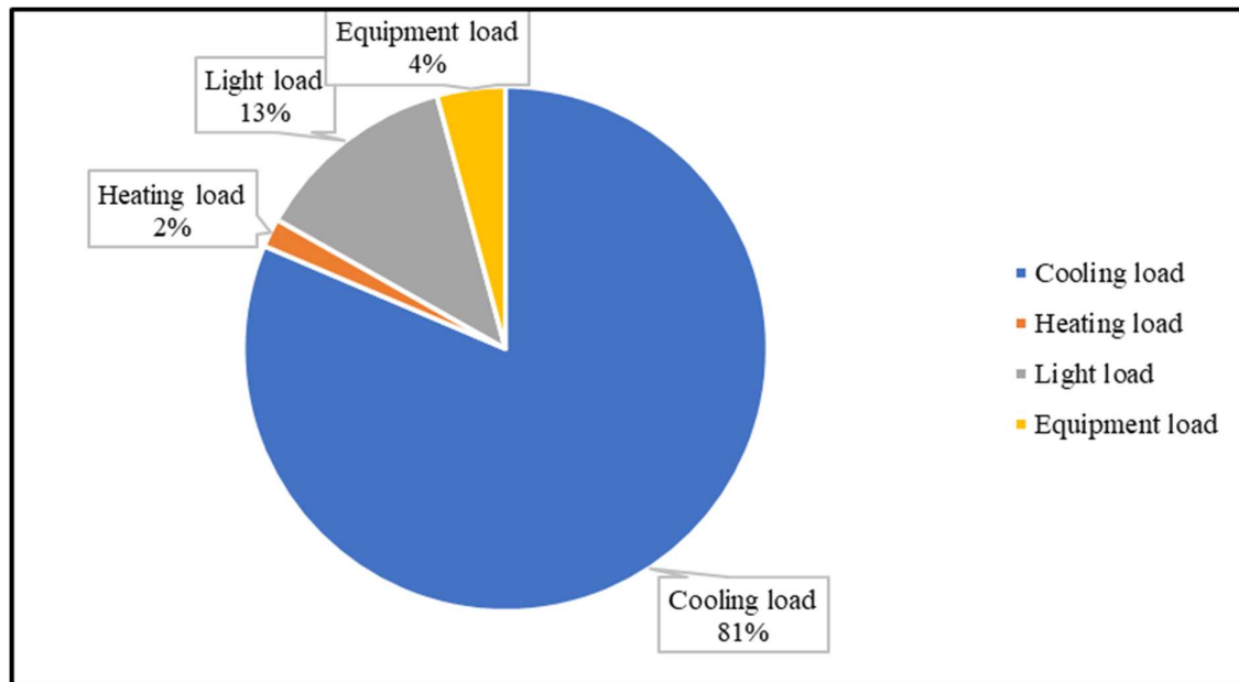
Fig. 9: Components of Predicted Annual Energy Consumption Using Revit (kWh)
