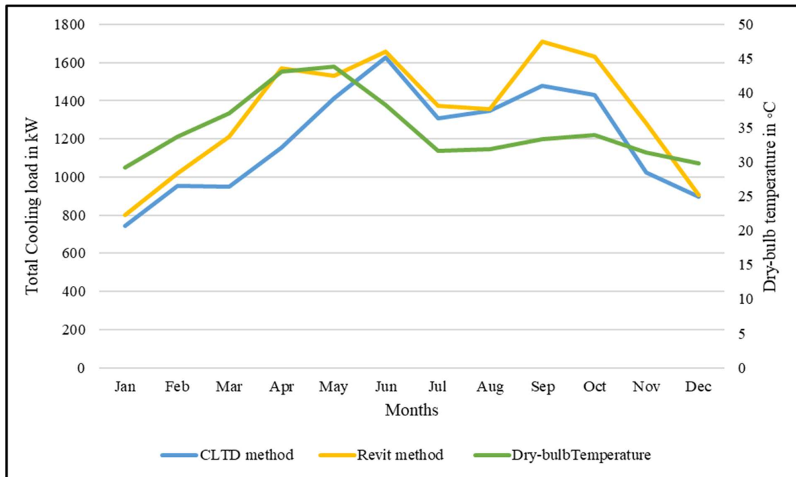
Fig. 8: Peak cooling load (KW) prediction by month for 2021
