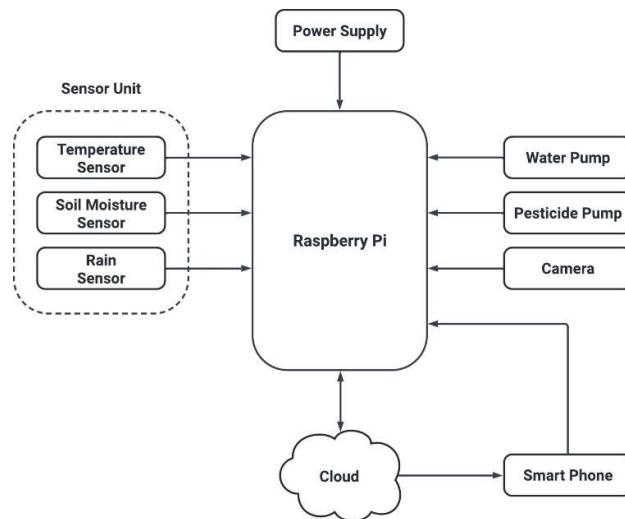
Fig. 6. System Architecture
