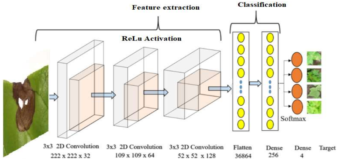
Fig.2. Proposed CNN Architecture
