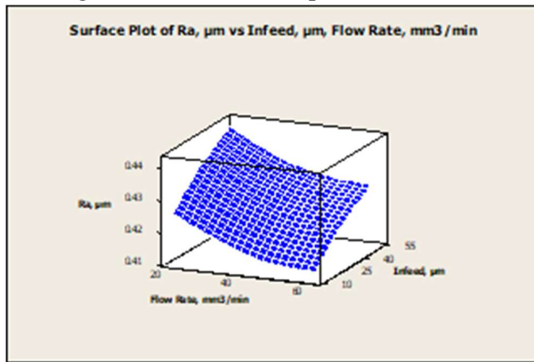
Fig.12. AISI 4340, Graphite as lubricant
