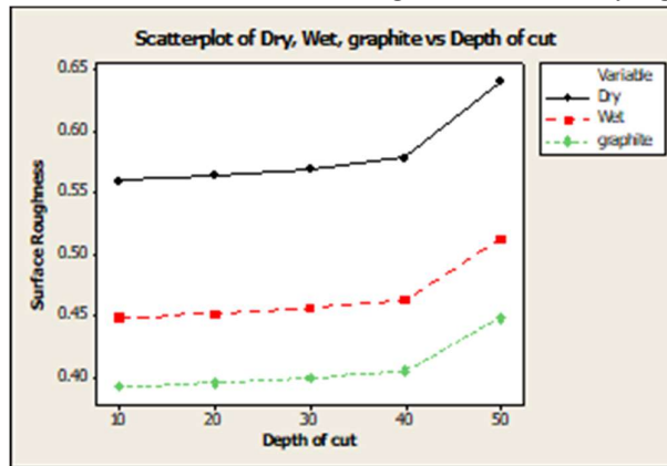
Fig. 3. Effect of coolants on Surface Roughness under varying depths of cut
