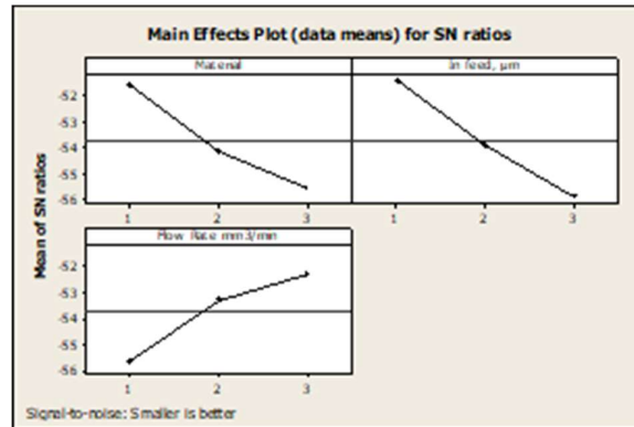
Fig.4. Main Effects Plot (Data Means) for SN ratios
