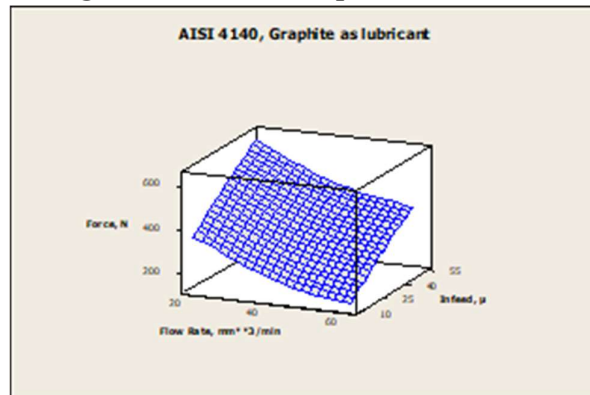
Fig.6. AISI 4140, Graphite as lubricant
