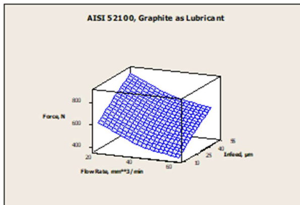
Fig. 8. AISI 52100, Graphite as lubricant
